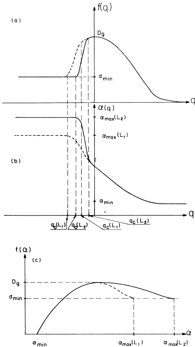
FIG. 1. Schematic dependence of (a) f(q, L) , (b) \alpha(q, L) , and (c) f(\alpha, L) , for a single growing aggregate at sizes L_1 (dashed line) and L_2 > L_1 (solid line). d_{\min} is the fractal dimension of the growth sites with the smallest growth probability. \alpha_{\max}(L) and q_0(L) are given in Eqs. (6) and (9).
