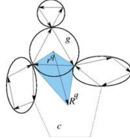
FIGURE 1. The vectors \vec{r}^q connect contacts around grain g . The vectors \vec{R}^q extend from grain centroids to cell centroid. These vectors are the diagonals of quadron q (blue).
