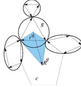
FIGURE 1. The vectors \vec{r}^q connect contacts around grain g . The vectors \vec{R}^q extend from grain centroids to cell centroid. These vectors are the diagonals of quadrangle q (blue).
