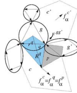
FIGURE 2. f_{\alpha}^q is the \alpha component of the loop force \vec{f}^c , which contains the quadron q (shaded blue). The loop forces of c and c' give the inter granular force at the contact point that they share, \vec{F}^{gg'} = \vec{f}^c - \vec{f}^{c'} [15]. Quadron p (striped) shares the same loop as q and hence also the same loop force.
